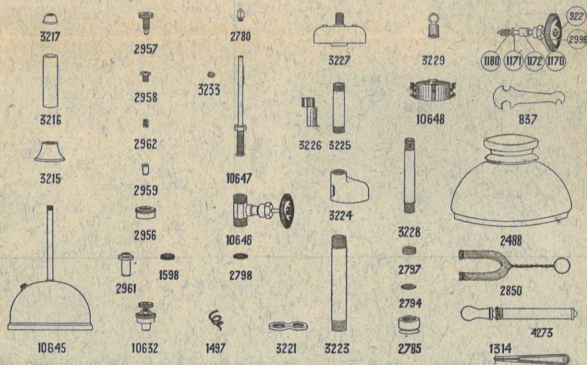
Lampes "Autolux" "Autolux" Lamps - Lamparas "Autolux"
